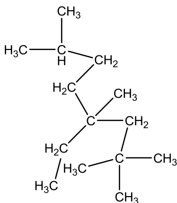
4-ethyl-2,2,4,7-tetramethyl-octaan
