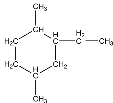
2-ethyl-1,4-dimethylcyclohexaan
