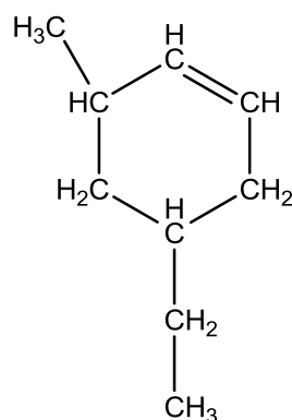
5-ethyl-3-methyl-cyclohexeen
