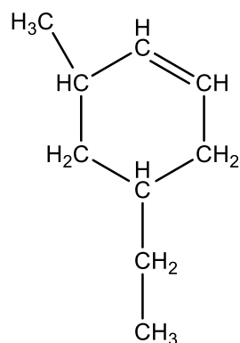
5-ethyl-3-methyl-cyclohexeen
